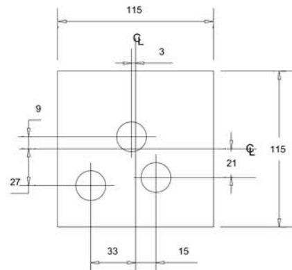
ITEM 7 HORIZONTAL LOCK 115 x 115 x 10 FLAT MACHINE CUT SQUARE NOT CROPPED
