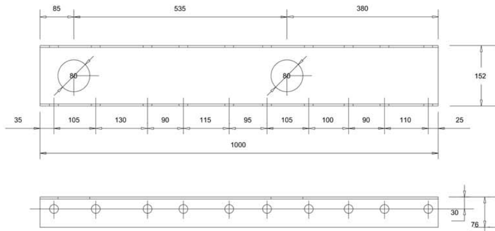
ITEM 1 VERTICAL CHANNELS 152 x 76 x 17.6kg /M 1000 LONG
