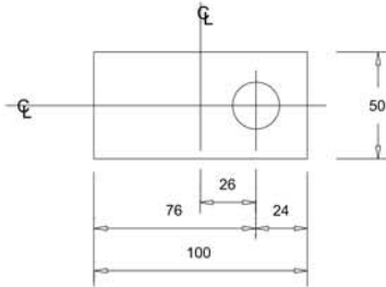
ITEM 5 SPACER 100 x 50 x 20 FLAT MACHINE CUT SQUARE NOT CROPPED
