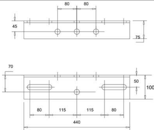
ITEM 2 POST ANGLE 100 x 75 x 8 ANGLE 440 LONG
