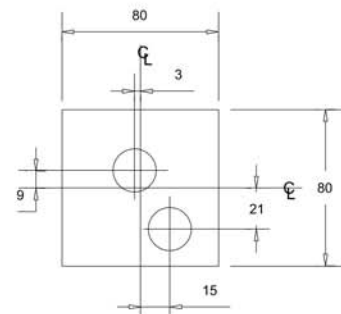
ITEM 6 VERTICAL LOCK 80 x 80 x 20 FLAT MACHINE CUT SQUARE NOT CROPPED
